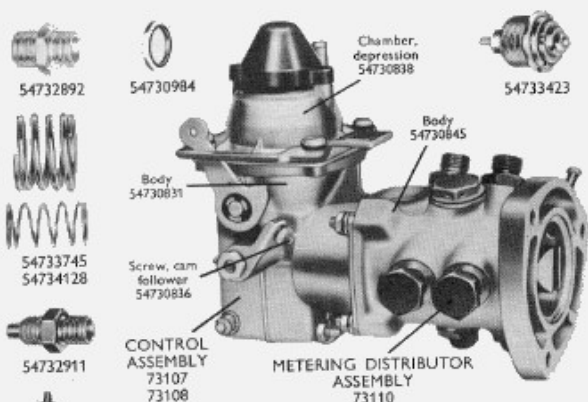
CONTROL AND METERING DISTRIBUTOR
