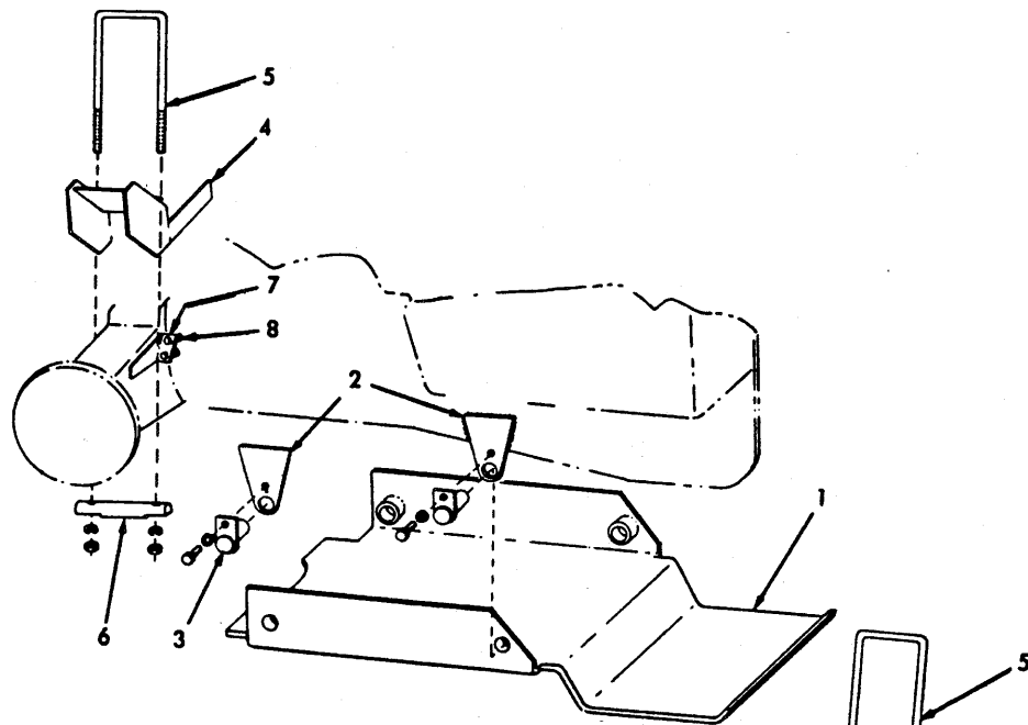
FRONT SECTION GUARDS
