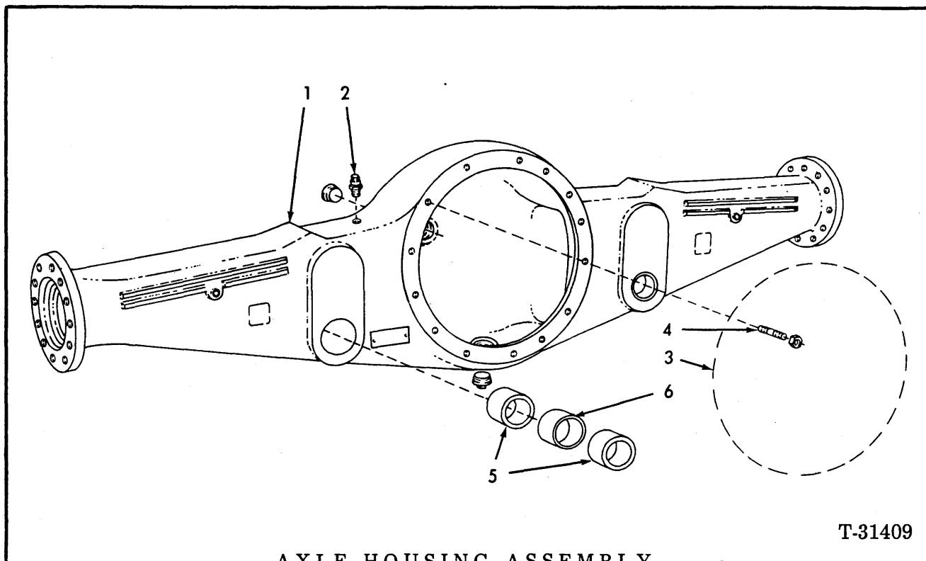
AXLE HOUSING ASSEMBLY (Rear Axle)
