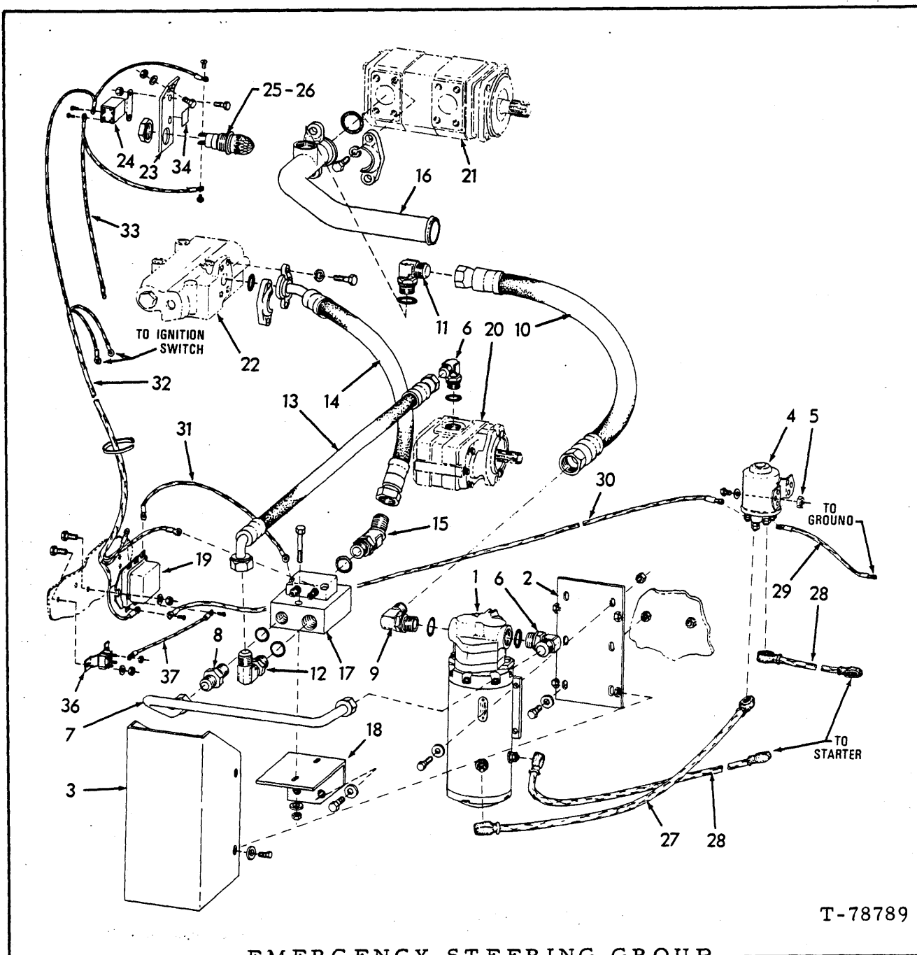
EMERGENCY STEERING GROUP
