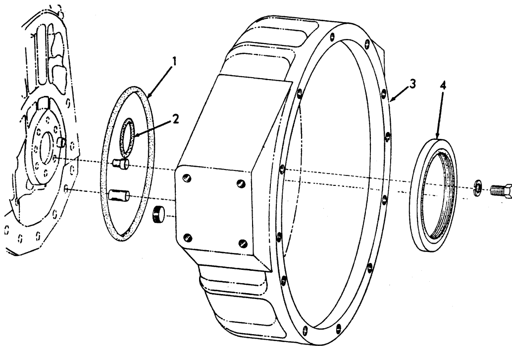
FLYWHEEL HOUSING
