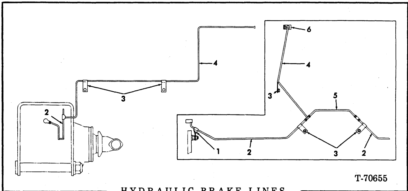
HYDRAULIC BRAKE LINES (Front Section)
