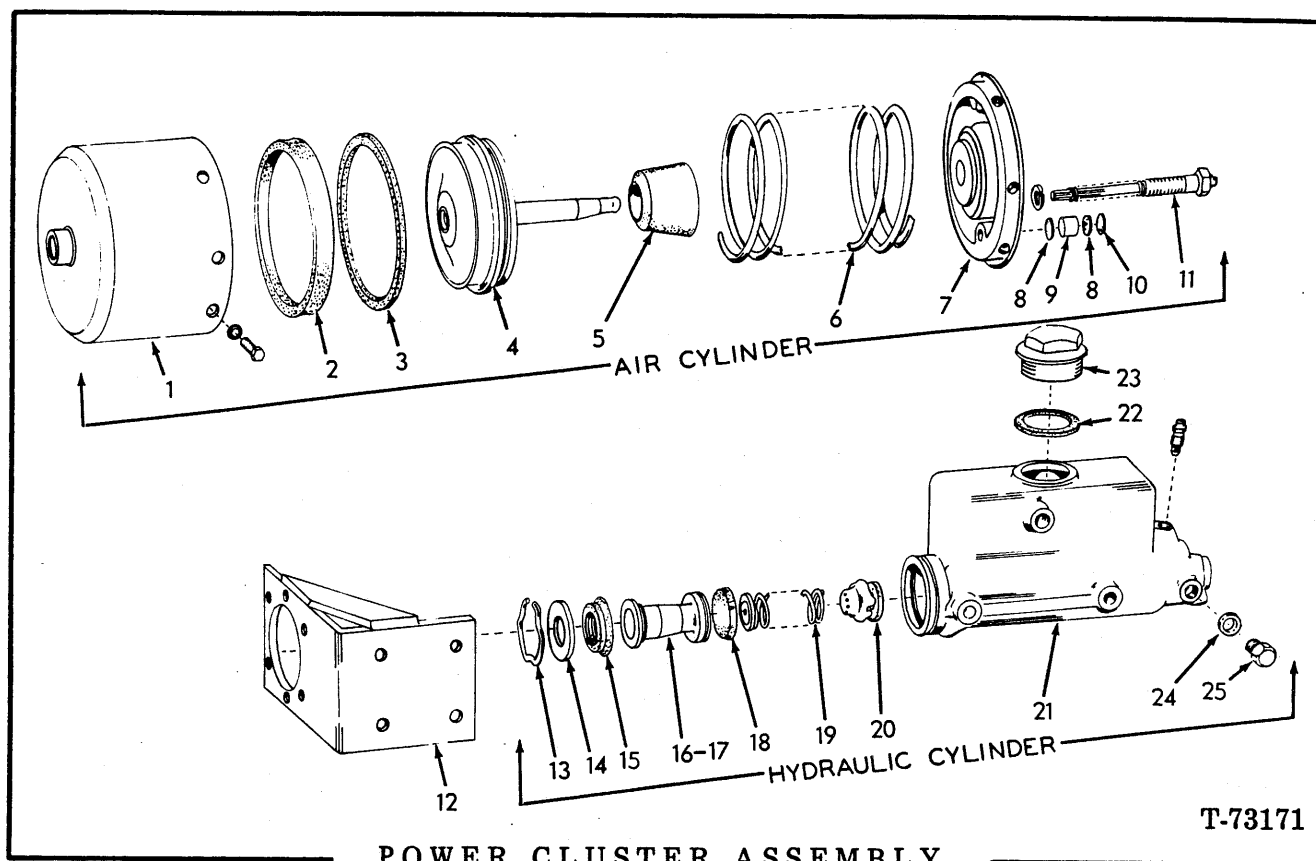
POWER CLUSTER ASSEMBLY
