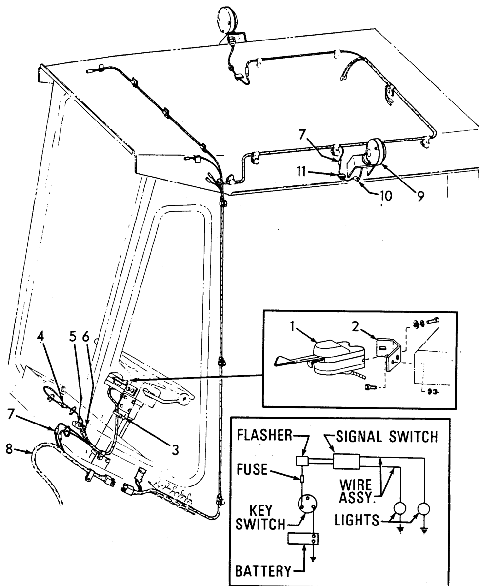
TURN SIGNALS (ROPS CAB)
