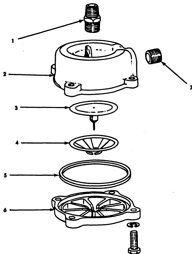
AIR TANK DRAIN VALVE (Moisture Ejector)
