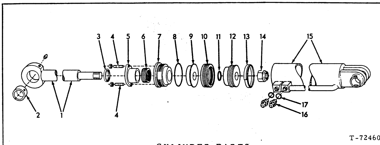
CYLINDER PARTS
