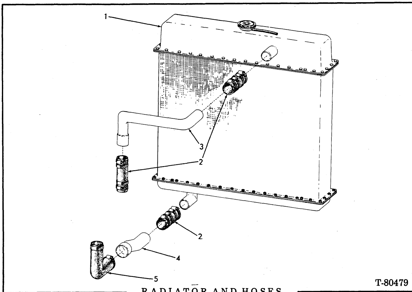
RADIATOR AND HOSES
