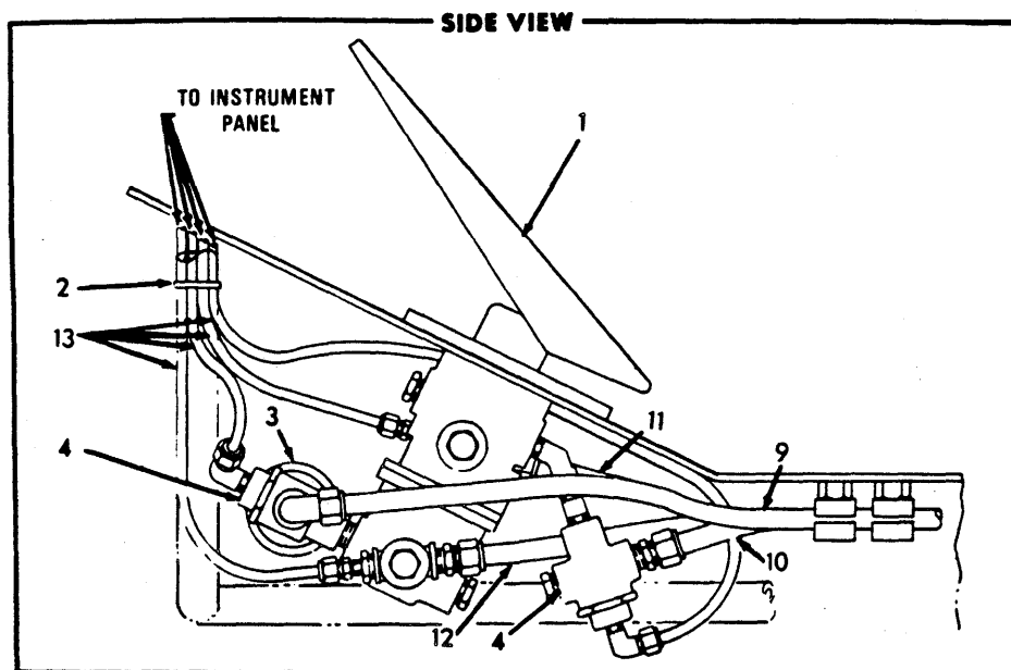
— AIR BRAKE LINES —
