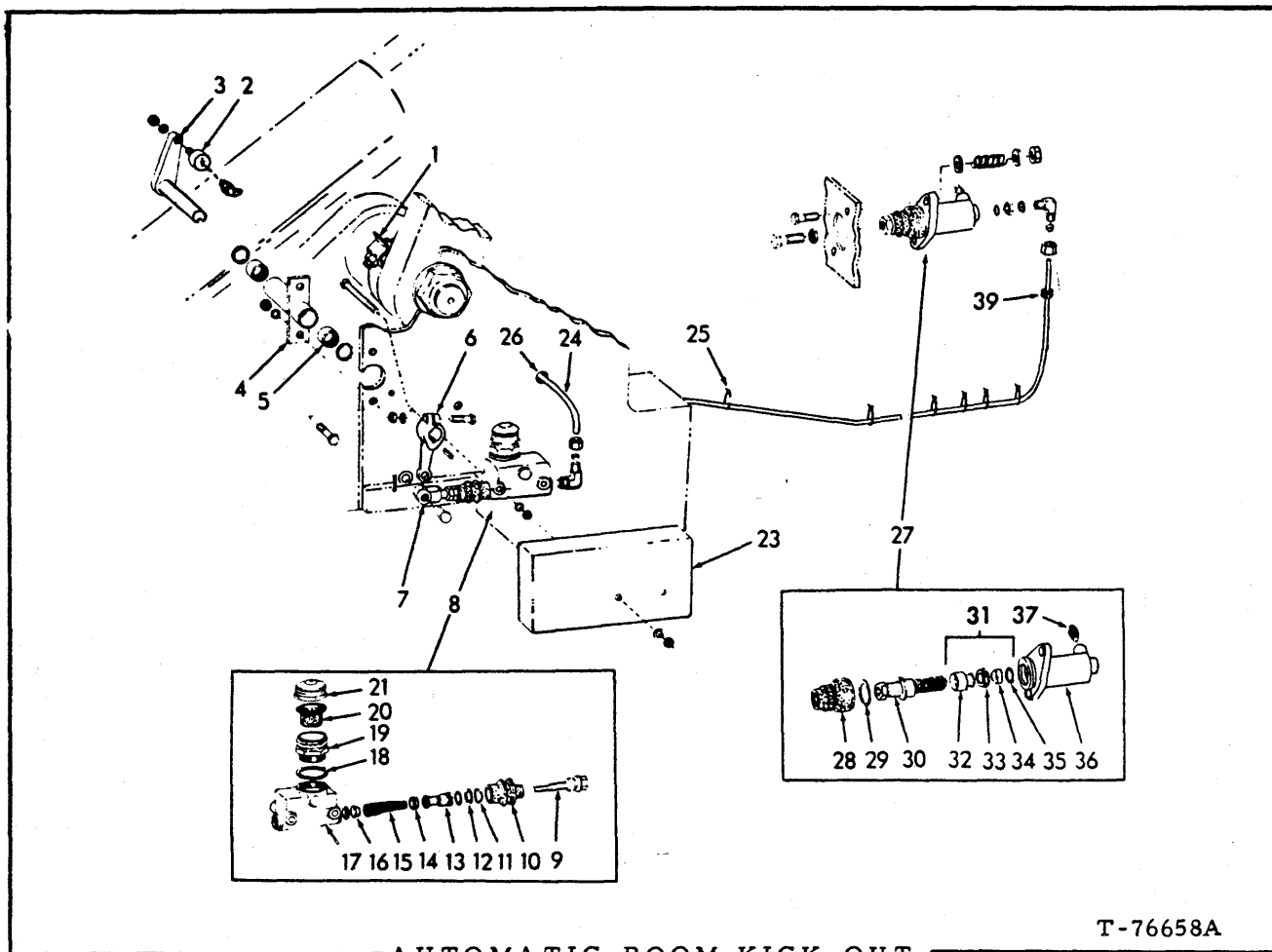
AUTOMATIC BOOM KICK-OUT (Single Lever Control)
