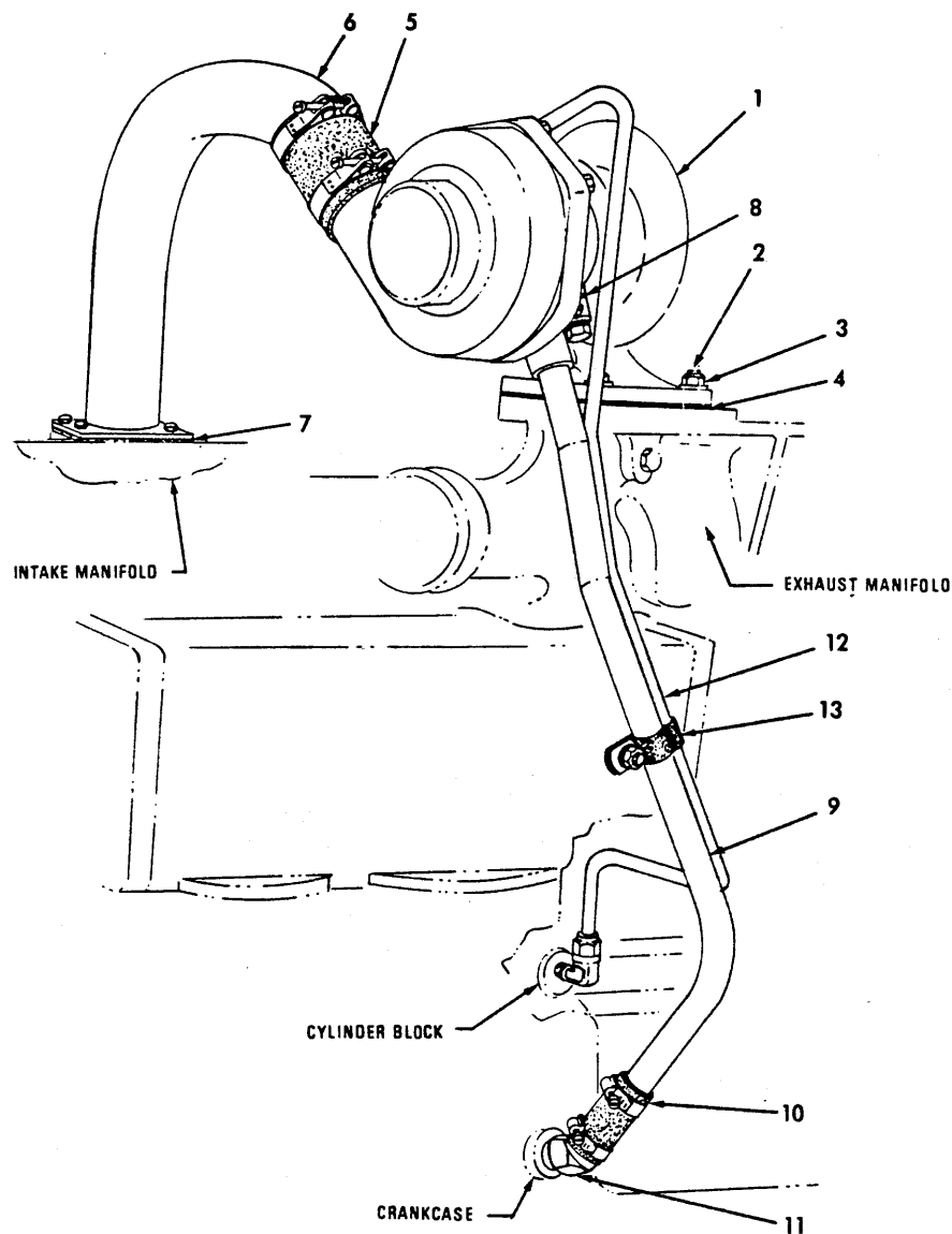
TURBOCHARGER (Airesearch)
