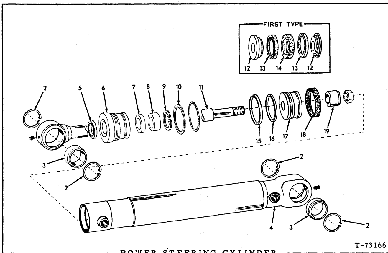
POWER STEERING CYLINDER
