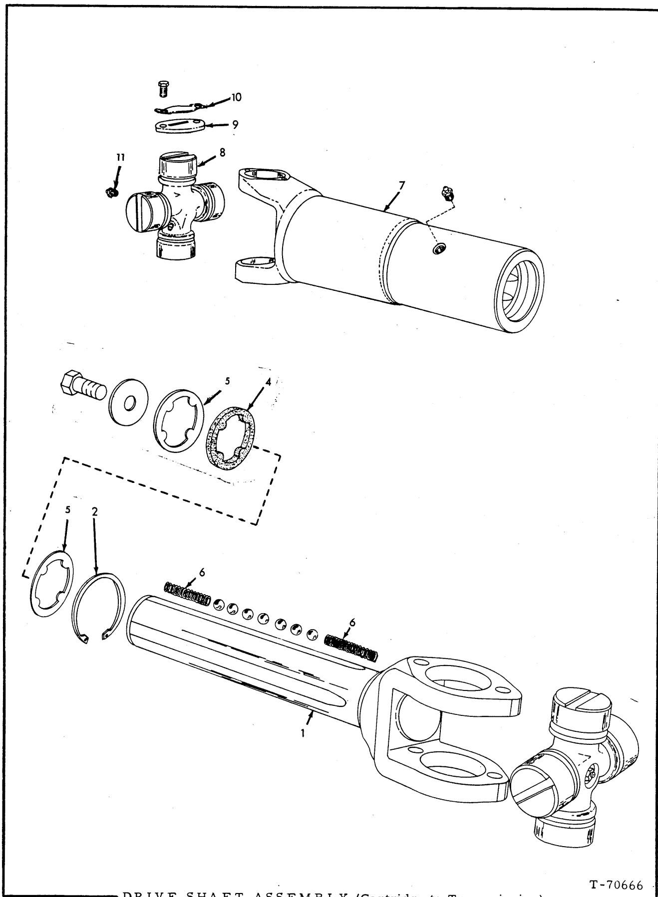
DRIVE SHAFT ASSEMBLY (Cartridge to Transmission)
