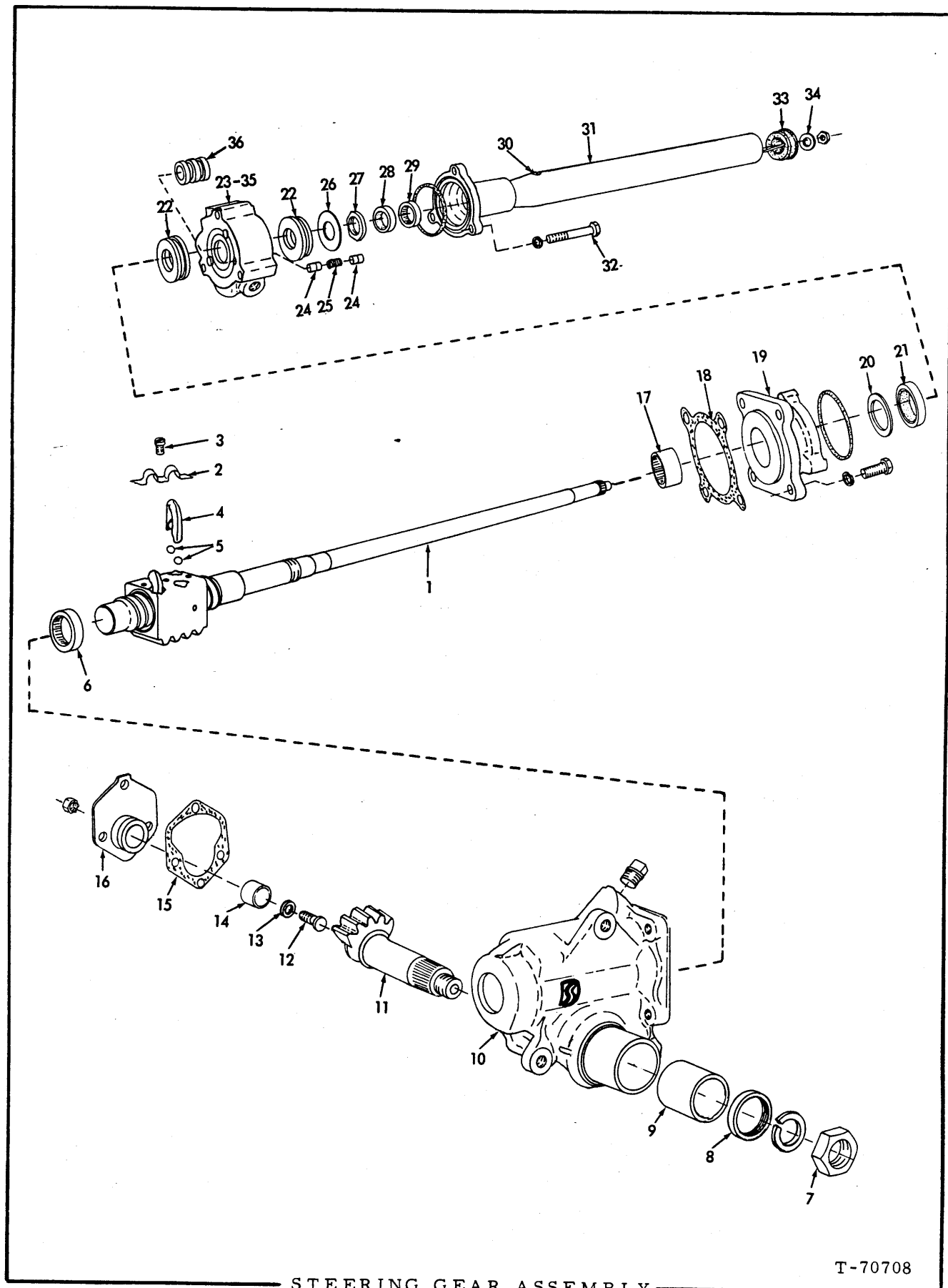
STEERING GEAR ASSEMBLY
