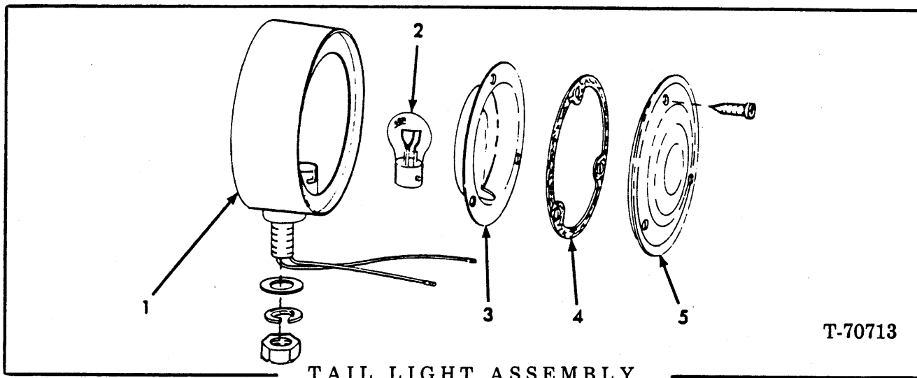
TAIL LIGHT ASSEMBLY
