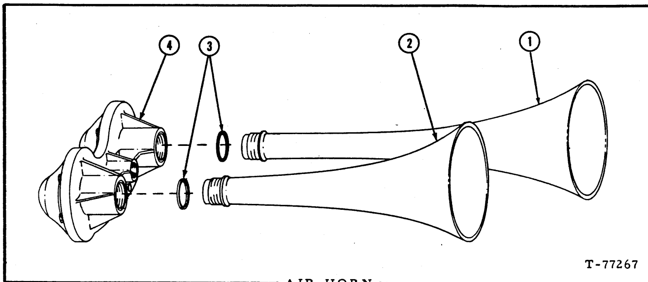
AIR HORN
