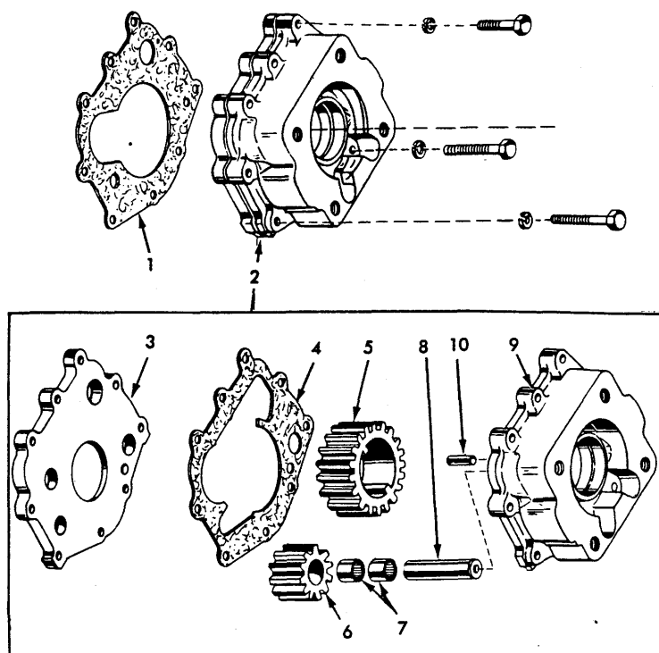
TRANSMISSION CHARGING OIL PUMP
