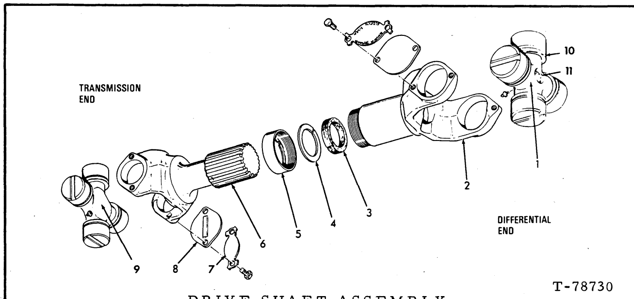
DRIVE SHAFT ASSEMBLY (Transmission to Rear Axle)
