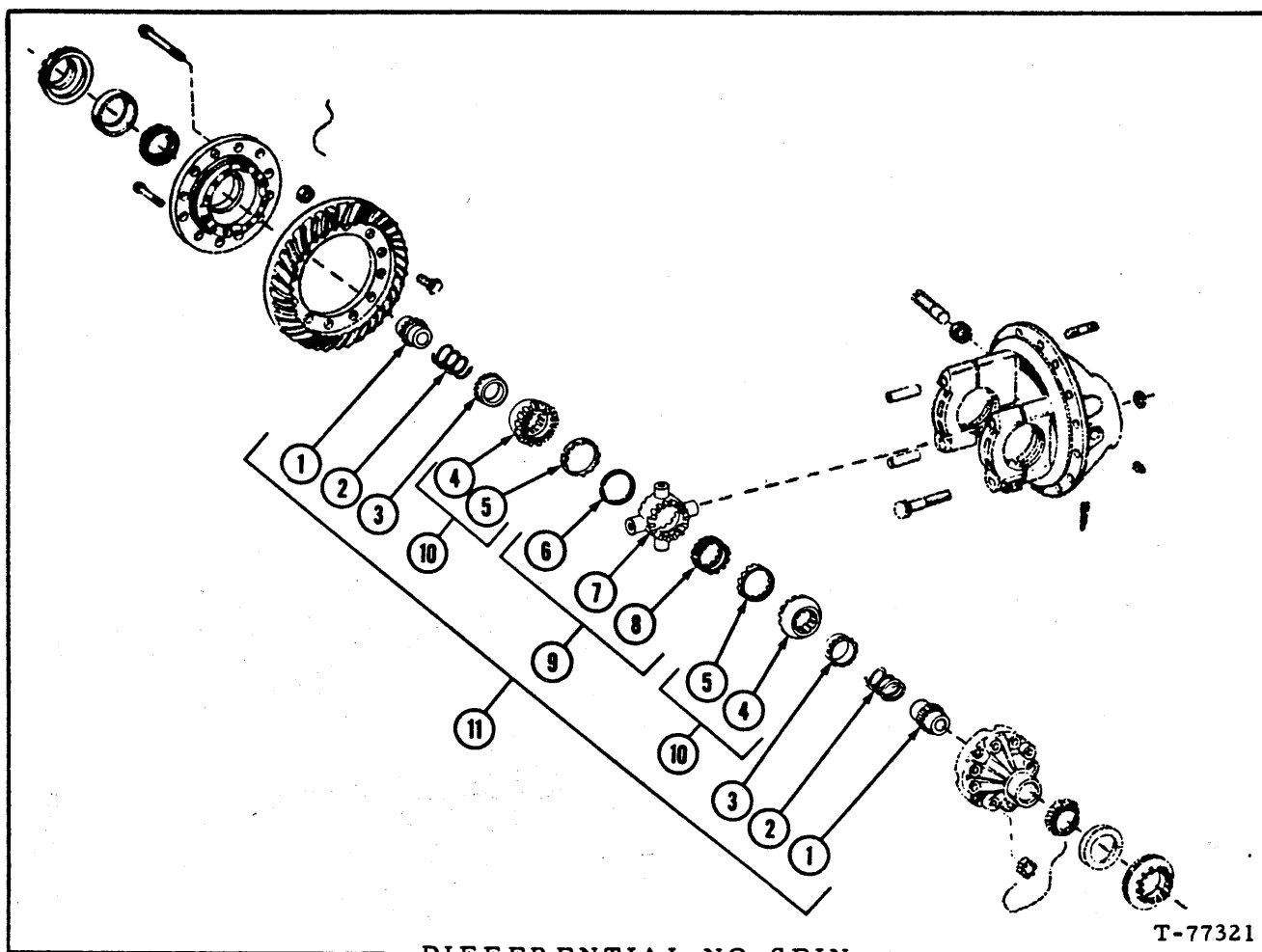
DIFFERENTIAL NO-SPIN (Rear Axle)
