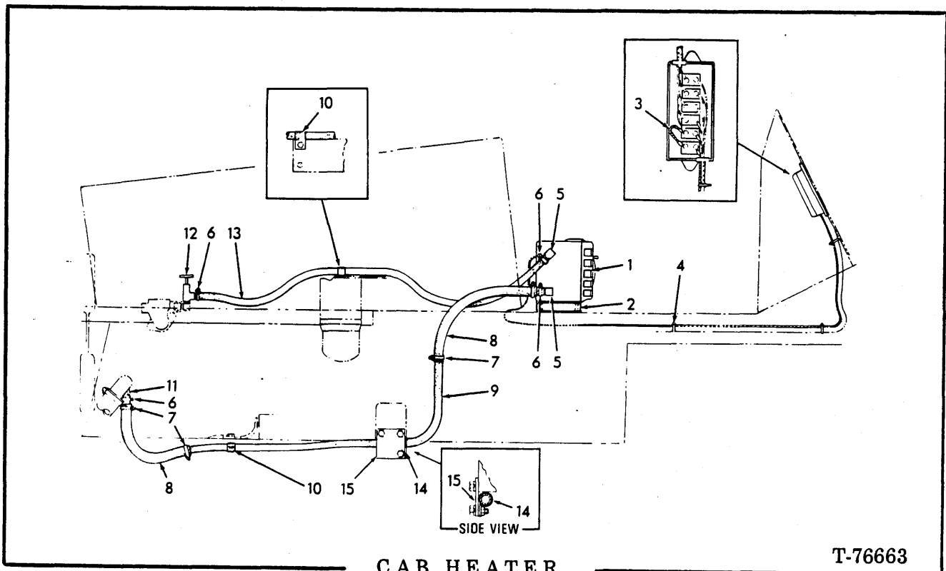
CAB HEATER
