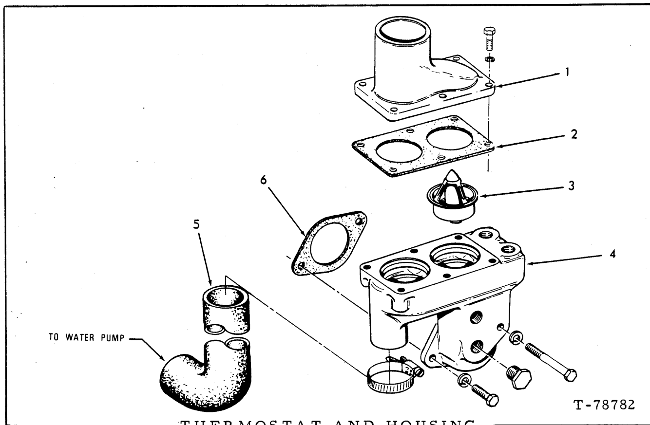
THERMOSTAT AND HOUSING
