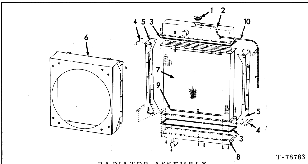
RADIATOR ASSEMBLY
