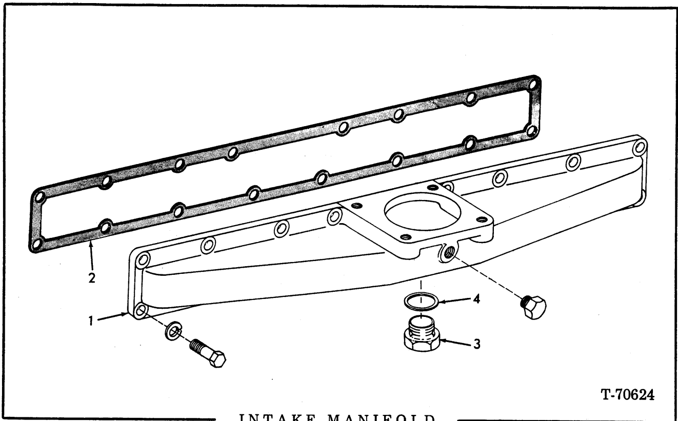
INTAKE MANIFOLD
