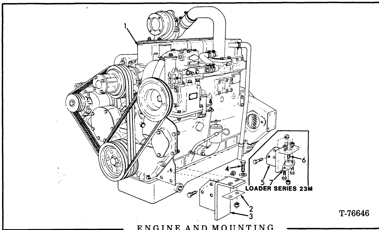
ENGINE AND MOUNTING
