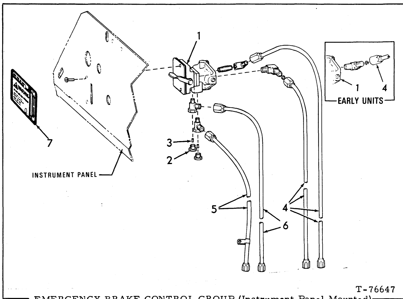
EMERGENCY BRAKE CONTROL GROUP (Instrument Panel Mounted)
