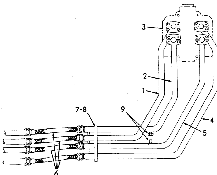
HYDRAULIC PIPING (Rear Section)
