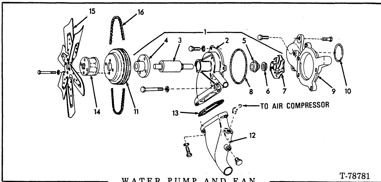
WATER PUMP AND FAN
