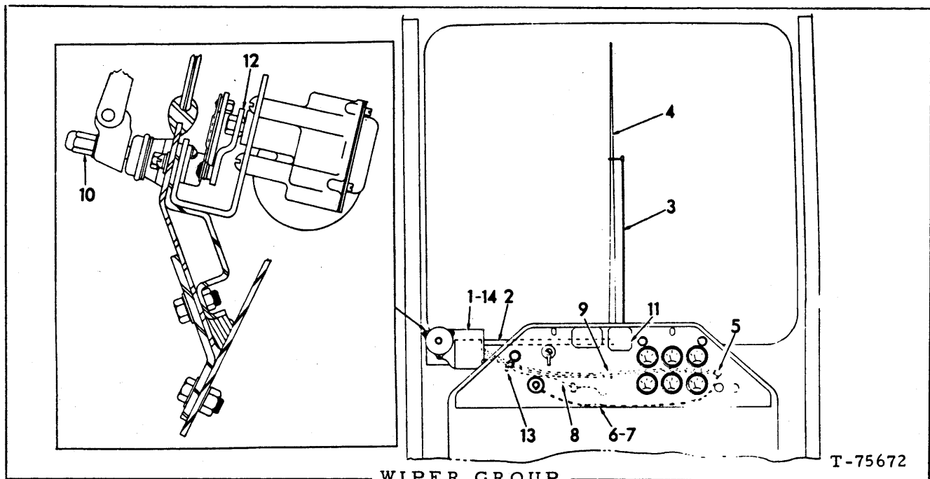
WIPER GROUP (Pantograph Wiper)
