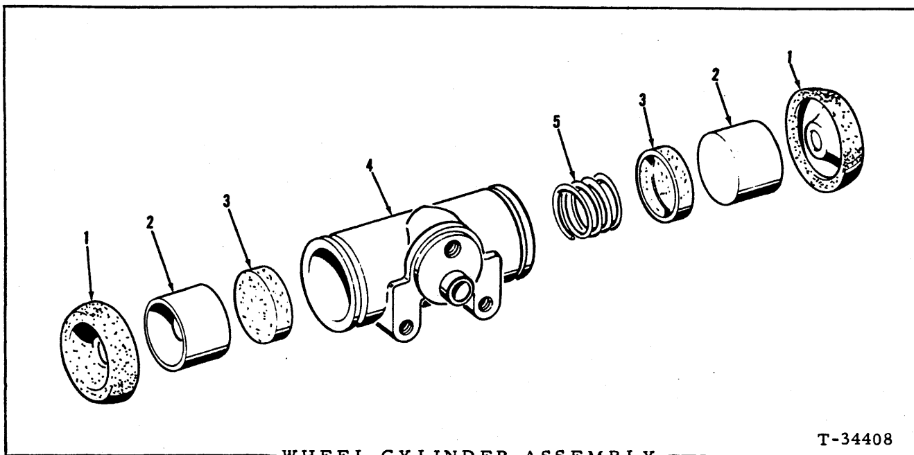
WHEEL CYLINDER ASSEMBLY
