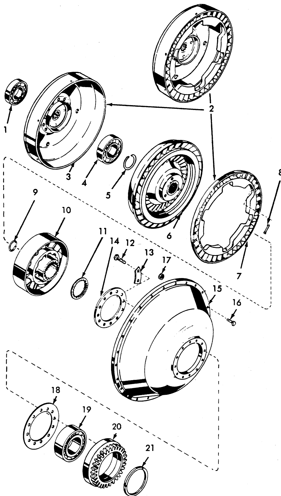
TORQUE CONVERTER
