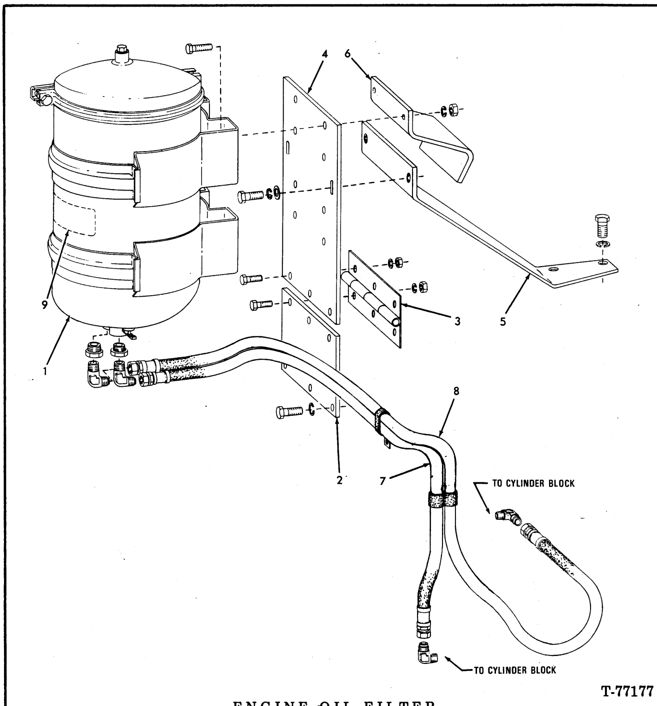
ENGINE OIL FILTER
