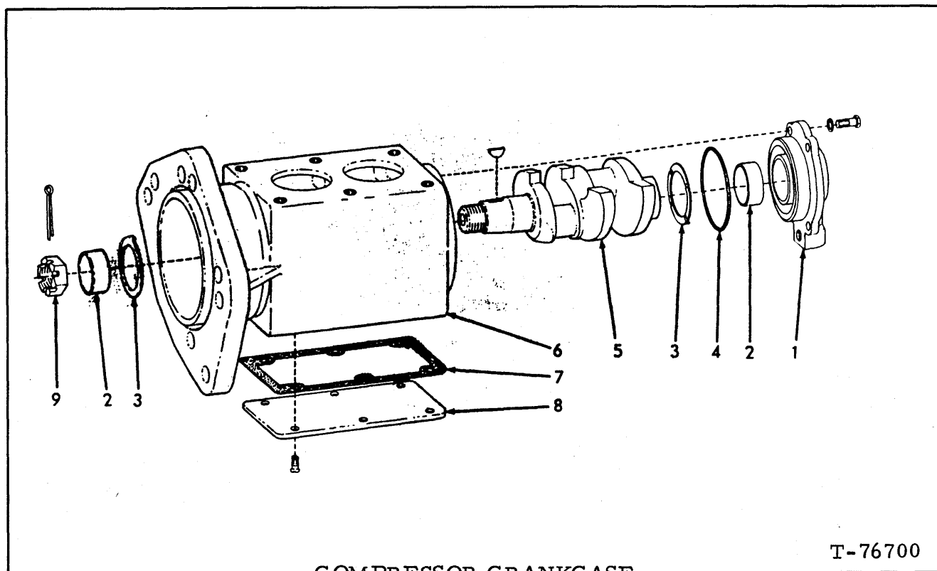
COMPRESSOR CRANKCASE
