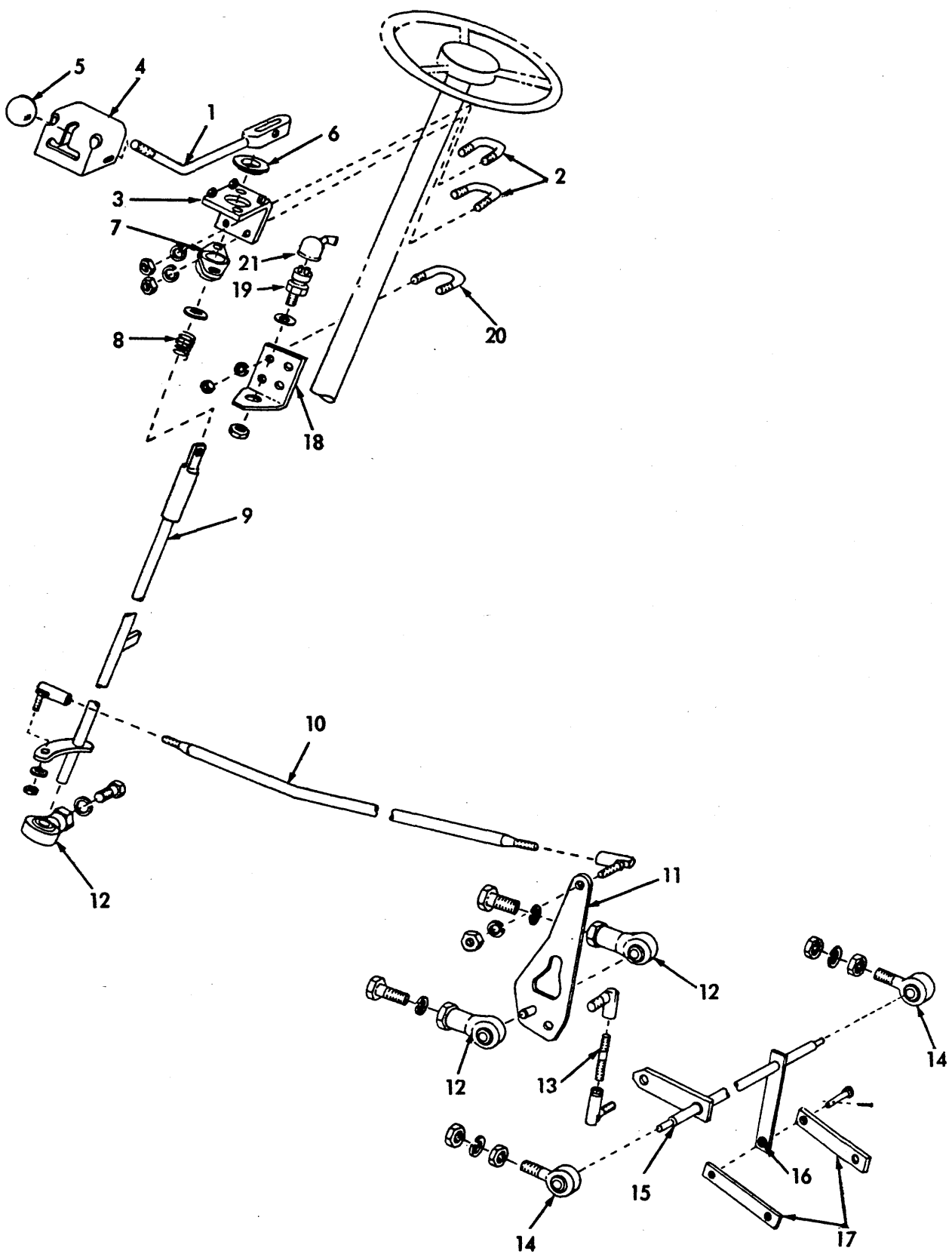
TRANSMISSION CONTROL GROUP
