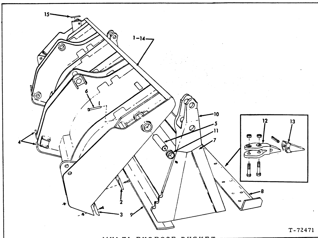
MULTI-PURPOSE BUCKET
