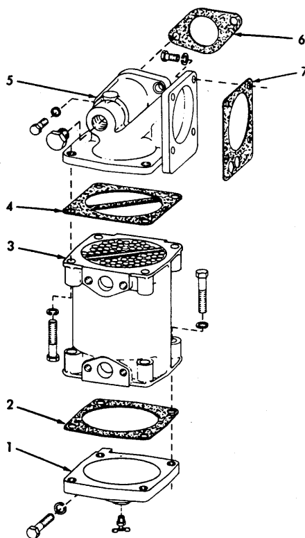
TRANSMISSION OIL COOLER
