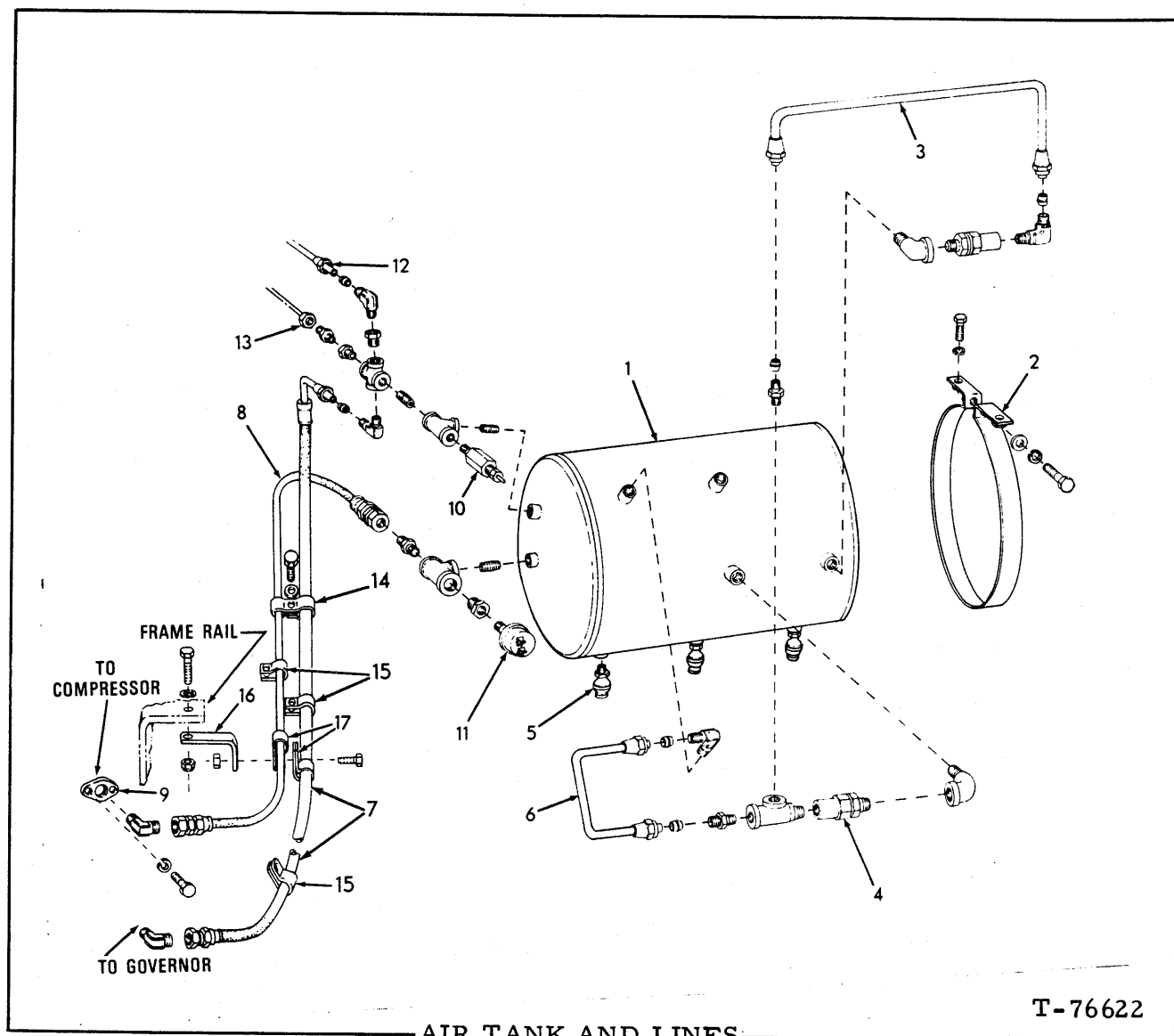
AIR TANK AND LINES
