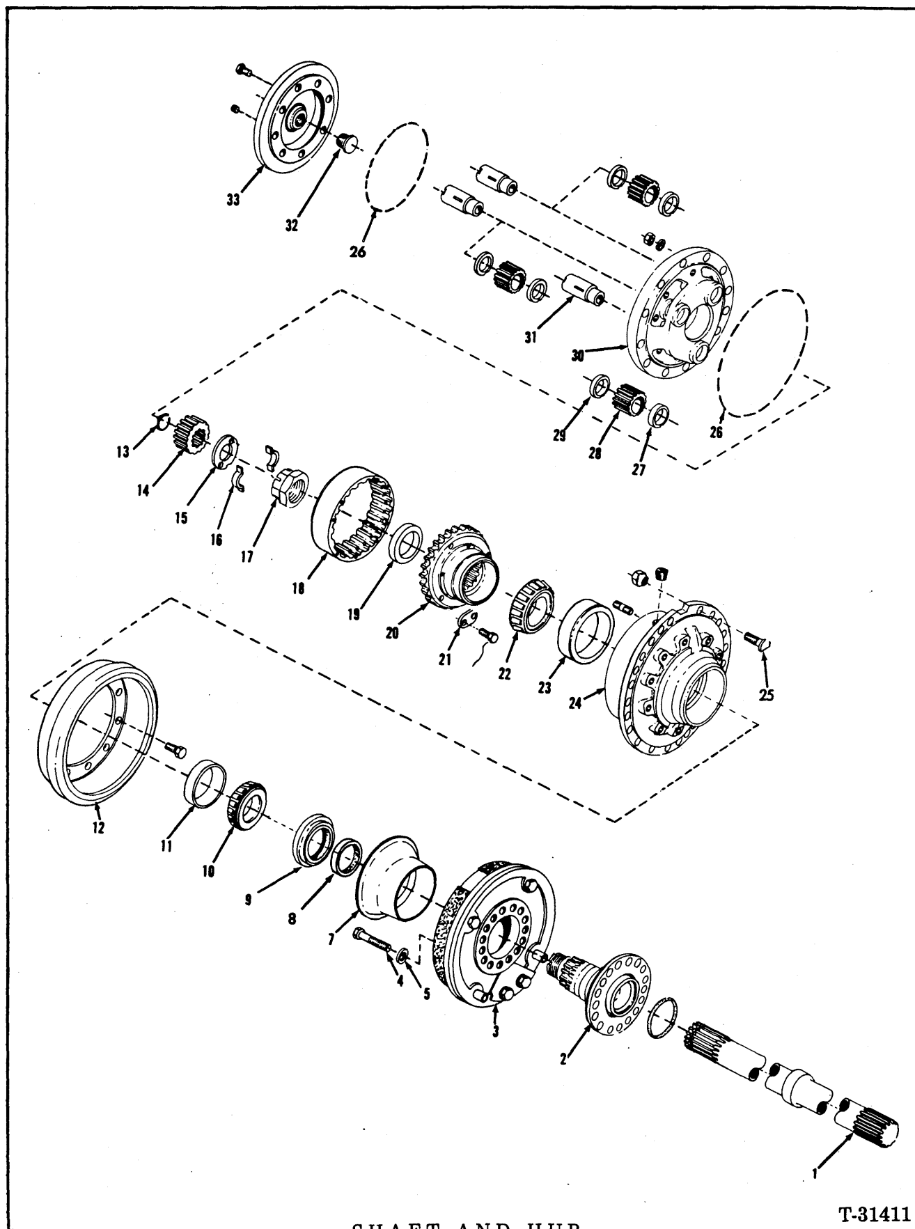
SHAFT AND HUB (Rear Axle)
