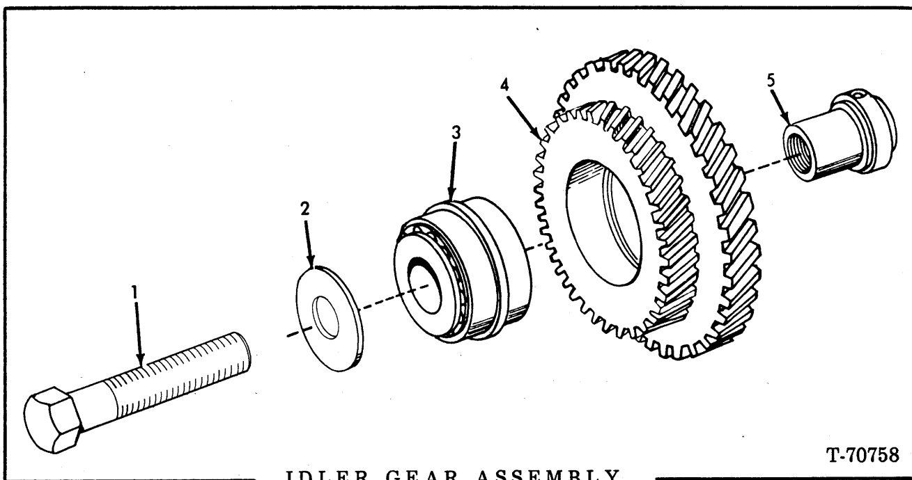
IDLER GEAR ASSEMBLY
