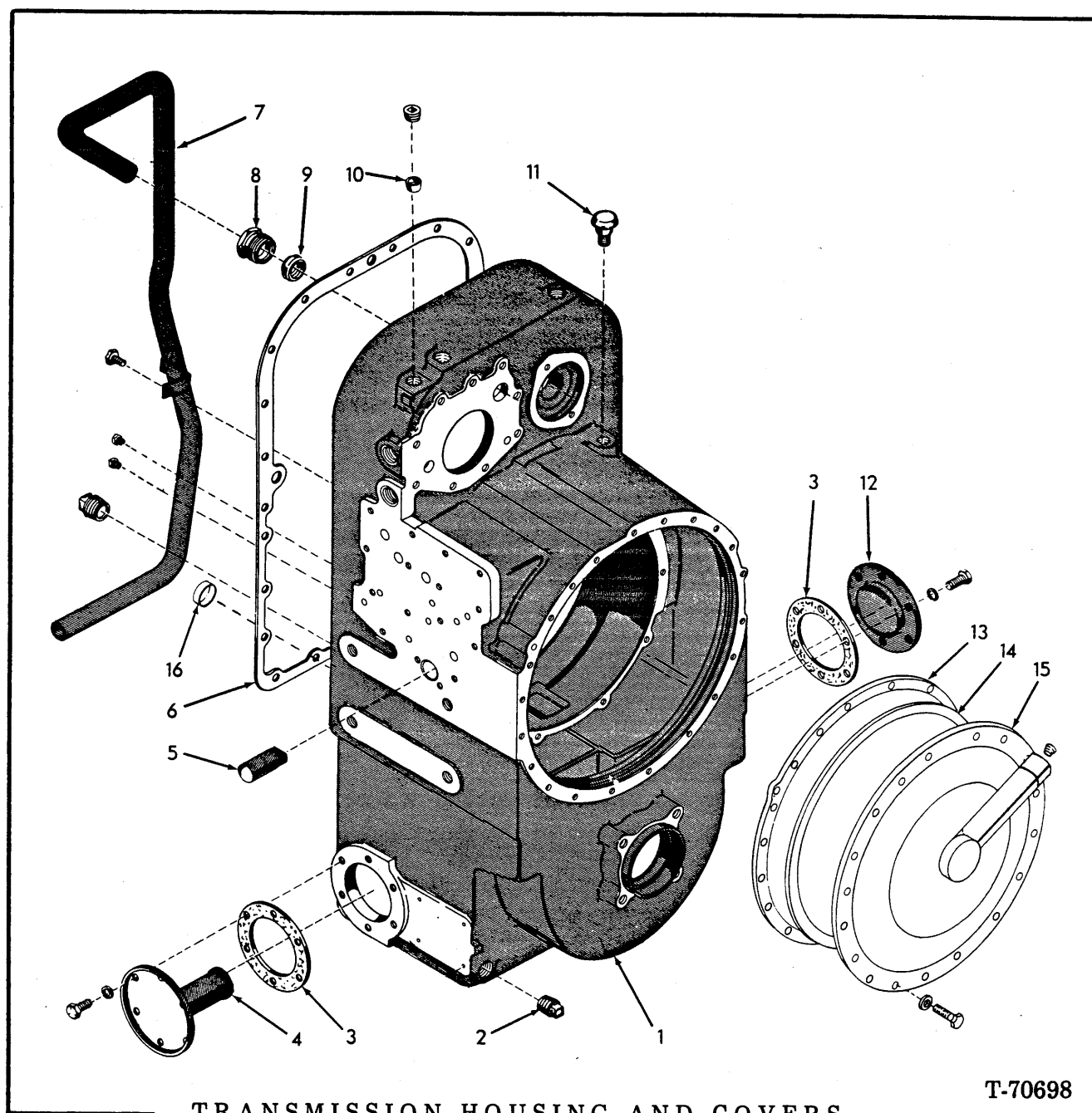
TRANSMISSION HOUSING AND COVERS
